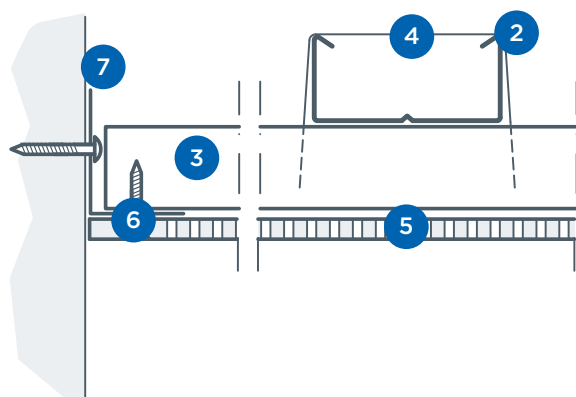
Detail B-B
